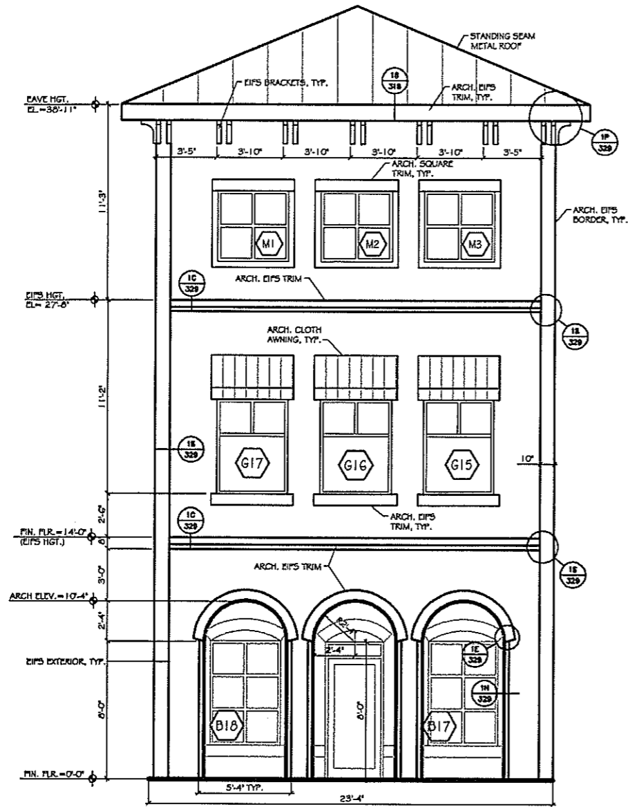
1 ENLARGED ELEVATION 320 SCALE 3/8" = 1'-0"
