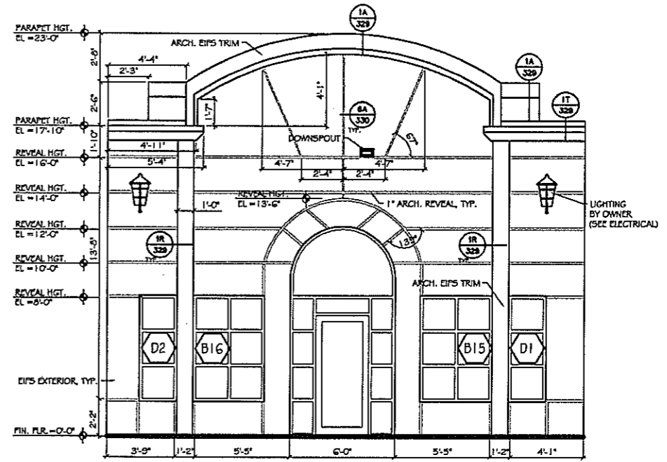
2 ENLARGED ELEVATION 320 SCALE 3/8" = 1'-0"
