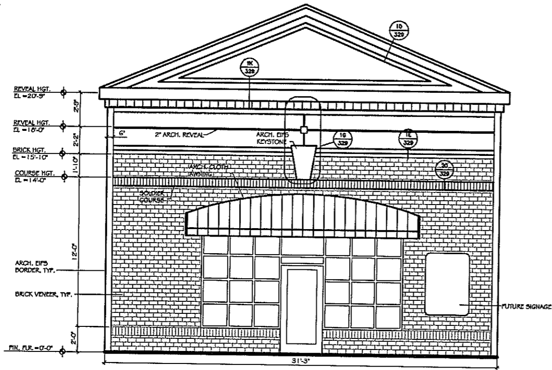
1 ENLARGED ELEVATION SCALE 3/8" = 1'-0"
