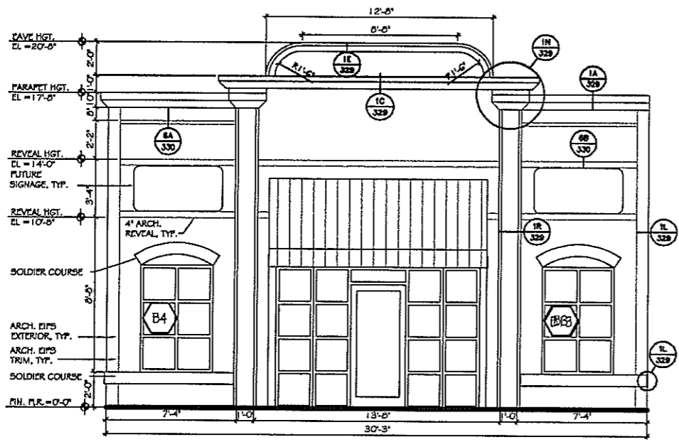
1 ENLARGED ELEVATION 322 SCALE 3/8" = 1'-0"
