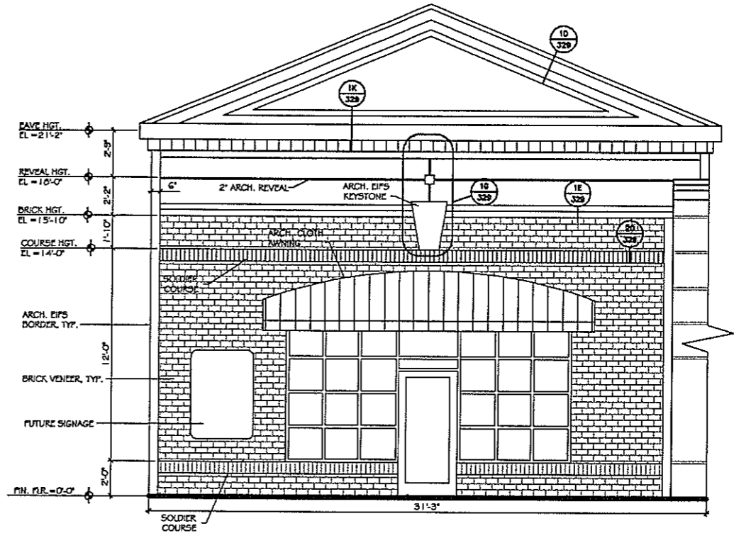
2 ENLARGED ELEVATION 322 SCALE 3/8" = 1'-0"
