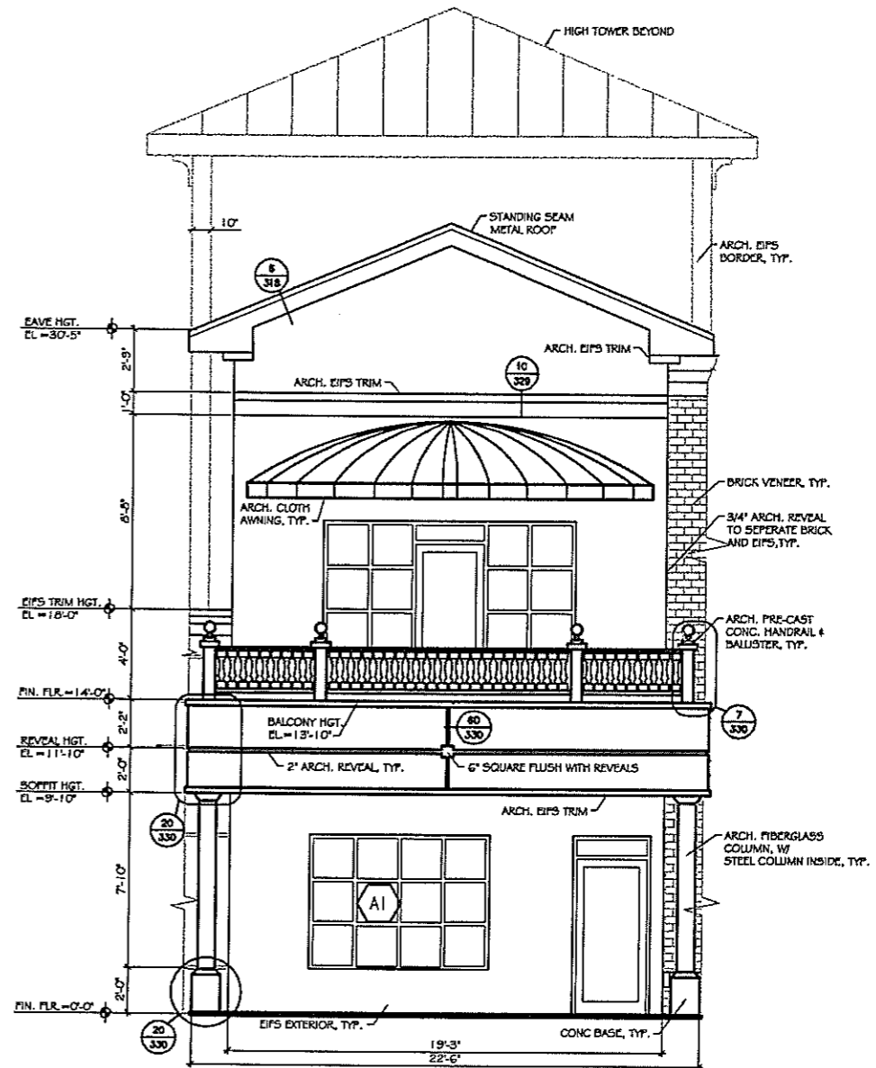
2 ENLARGED ELEVATION SCALE 3/8" = 1'-0"
