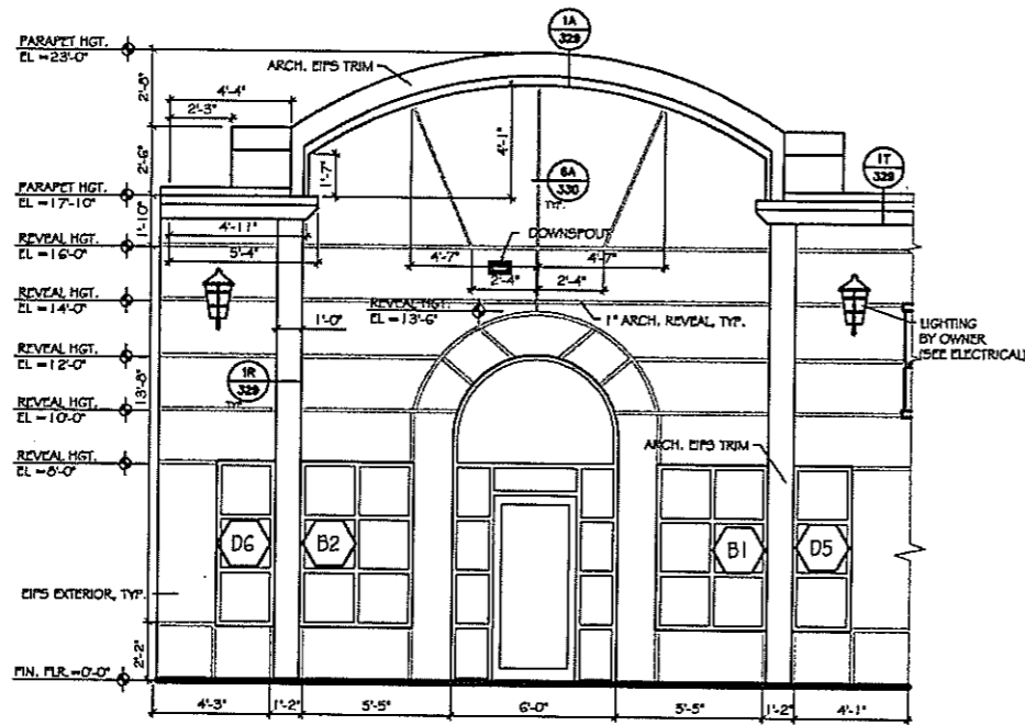
1 ENLARGED ELEVATION SCALE 3/8" = 1'-0"
