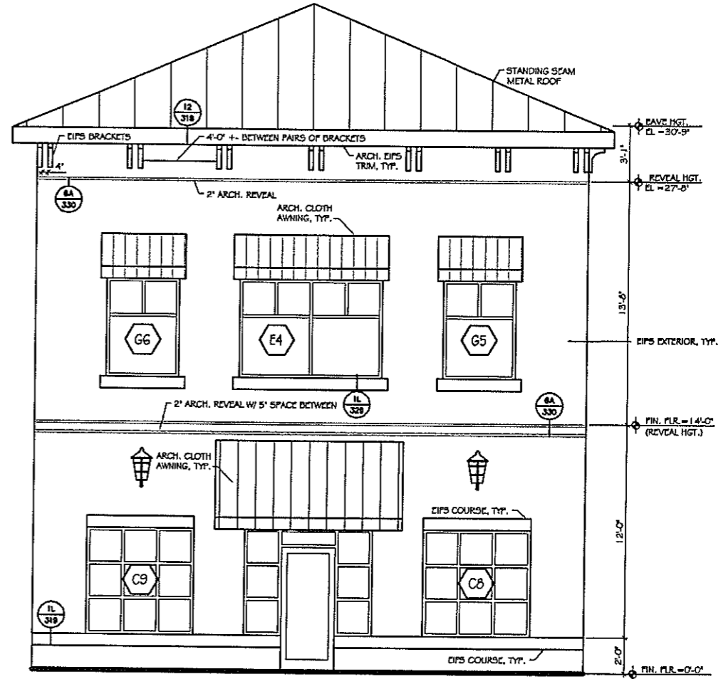
2 ENLARGED ELEVATION 324 SCALE 3/8" = 1'-0"
