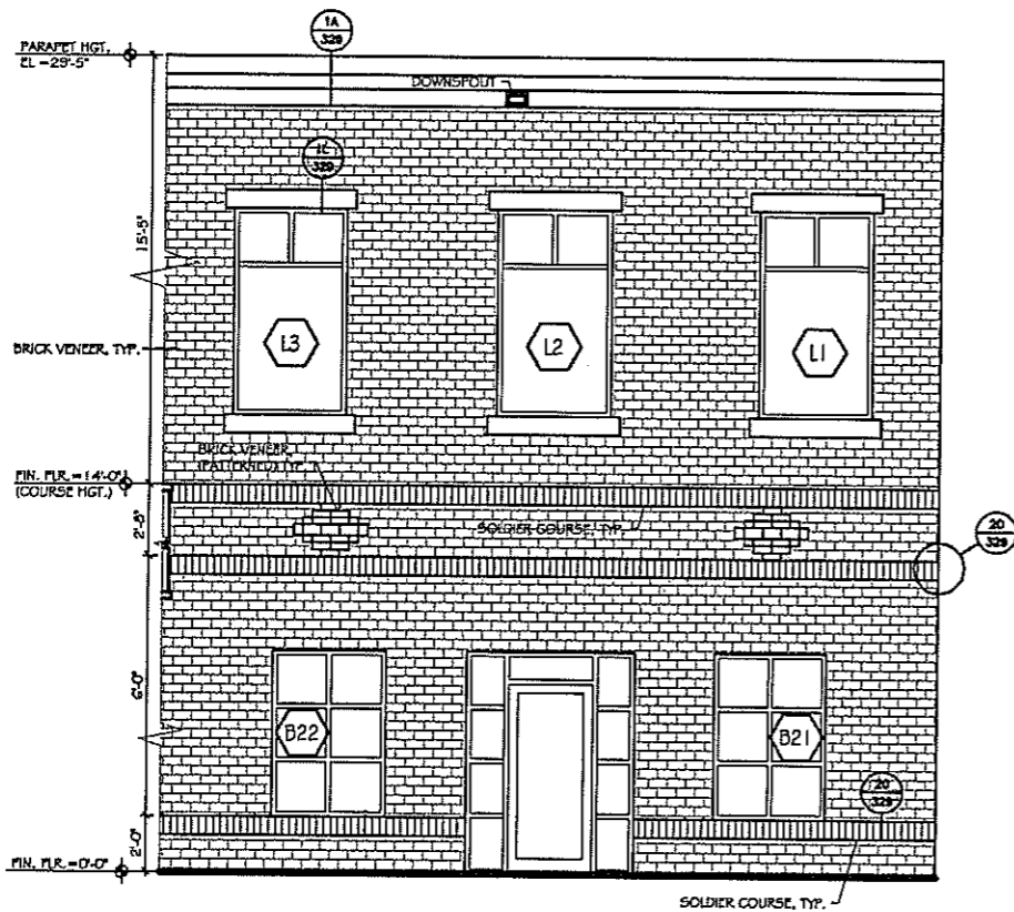
1 ENLARGED ELEVATION 324 SCALE 3/8" = 1'-0"
