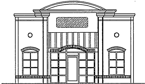
WEST ELEVATION
