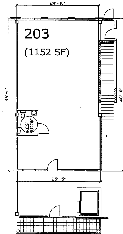
FLOOR PLAN
