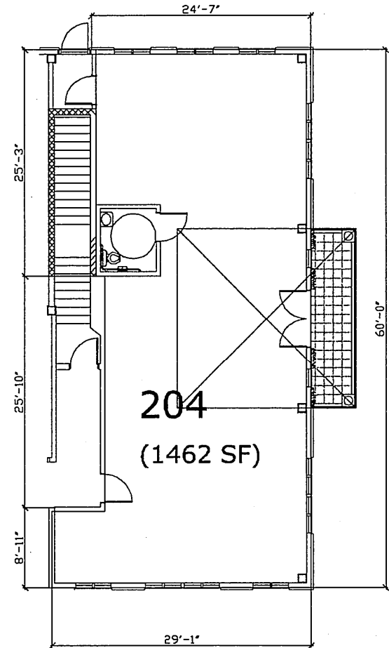
FLOOR PLAN
