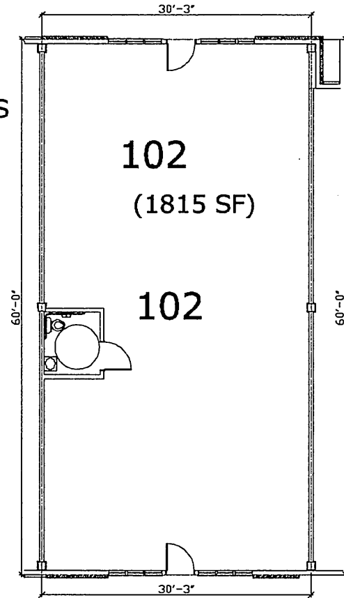
FLOOR PLAN
