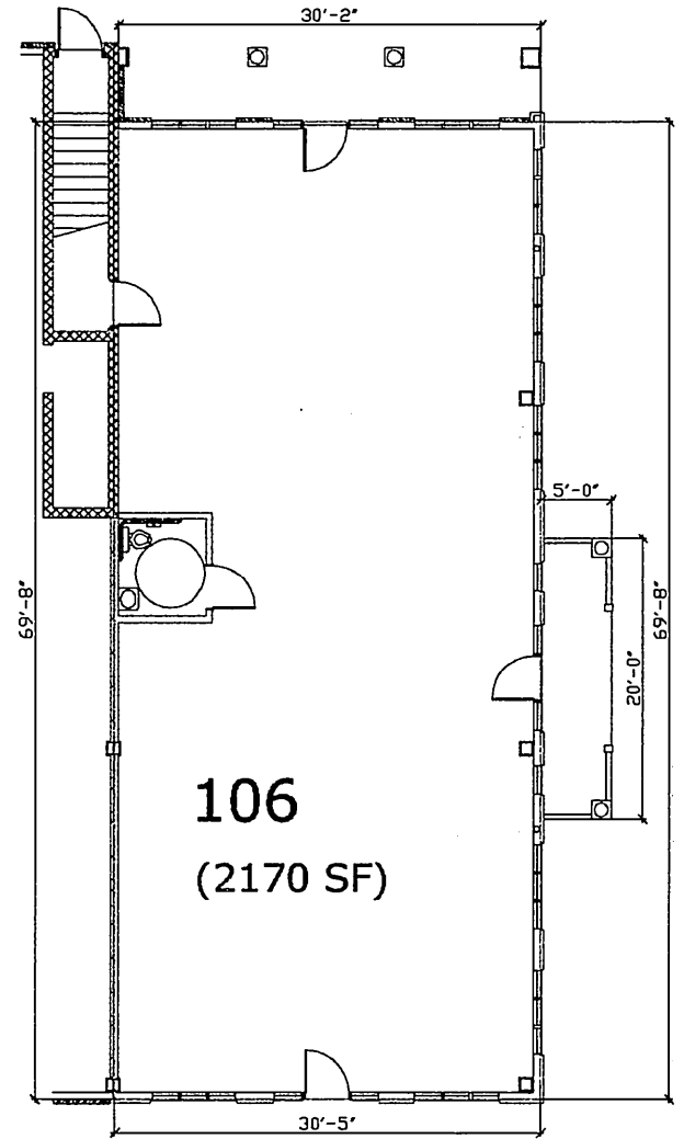
FLOOR PLAN
